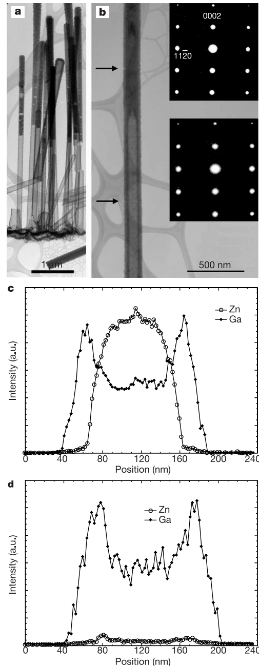
Figure 4 Characterization of the interface between the GaN tube and the ZnO wire. a, b , TEM images of arrays of GaN nanotubes with their ZnO nanowire templates partially removed. Insets in b are electron-diffraction patterns recorded on the core–sheath and the pure tube region along the [\bar{1}10] zone axis. c, d , Compositional (Ga and Zn signals) line profiles for core–sheath GaN/ZnO ( c ) and the GaN tube region ( d ) indicated by upper and lower arrows in b , respectively.
