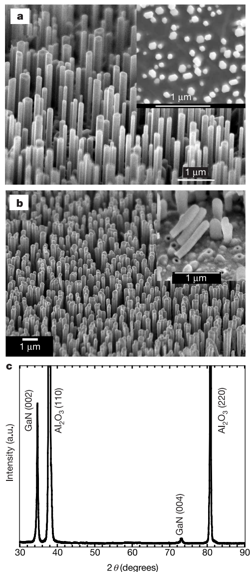
Figure 1 Arrays of ZnO nanowires and GaN nanotubes. Shown are SEM images of the ZnO nanowire template arrays (a), and the resulting GaN nanotube array (b). Inset in a shows cross-sections of the ZnO nanowires. Inset in b shows the fractured interface between the GaN nanotubes and the substrate. c, XRD of the GaN nanowire array.
