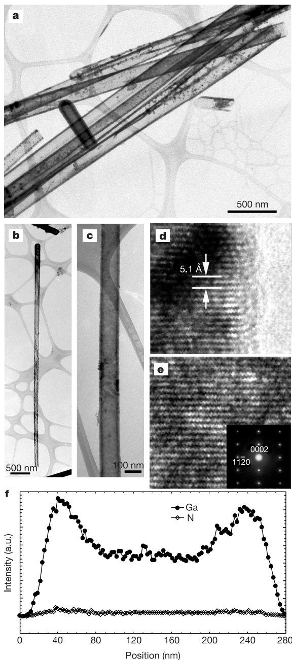
Figure 2 Structural characterization of GaN nanotubes. a–c, TEM images of the GaN nanotubes (a–c). d, High-resolution TEM images of a GaN nanotube wall at the surface, and e, the inside of the tube. Inset in e is an electron-diffraction pattern of the nanotube along the [\bar{1}10] zone axis. f, Compositional line profile across the nanotube probed by EDX spectroscopy.
