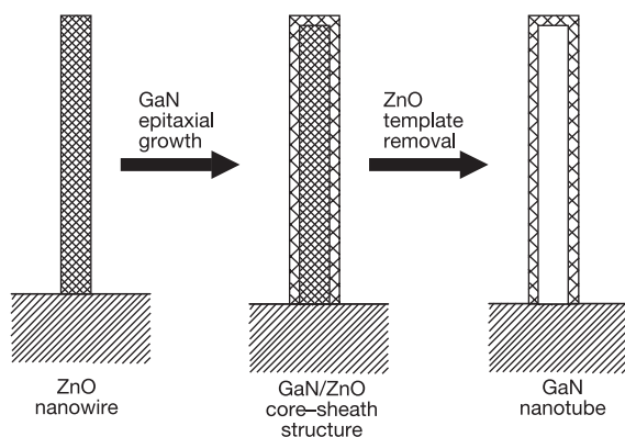
Figure 3 Schematic illustration of the ‘epitaxial casting’ process for making single-crystal GaN nanotubes.
